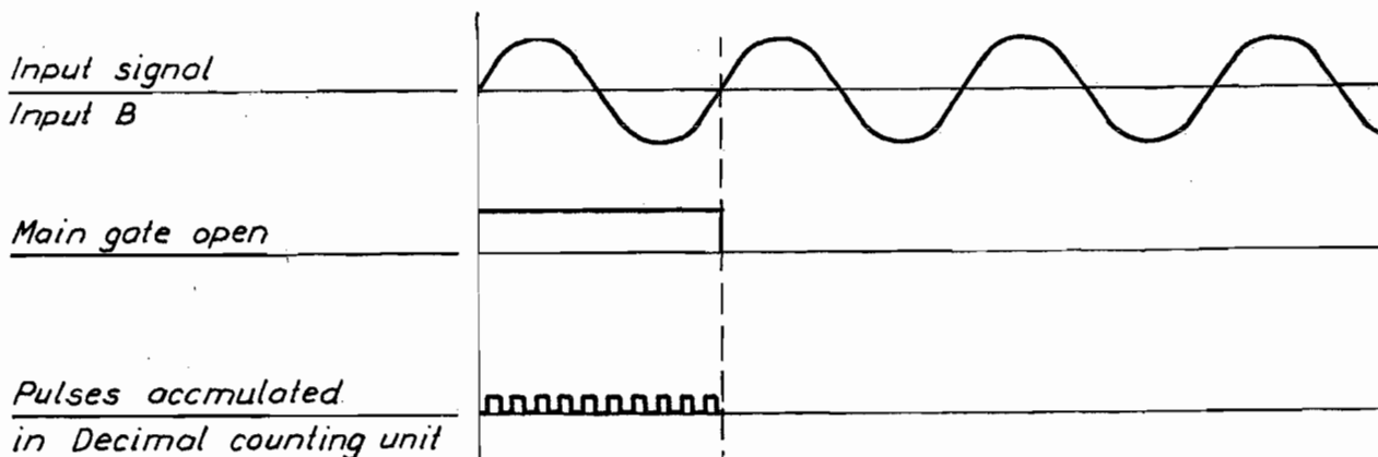
Fig. VI-7. Single period measurement
