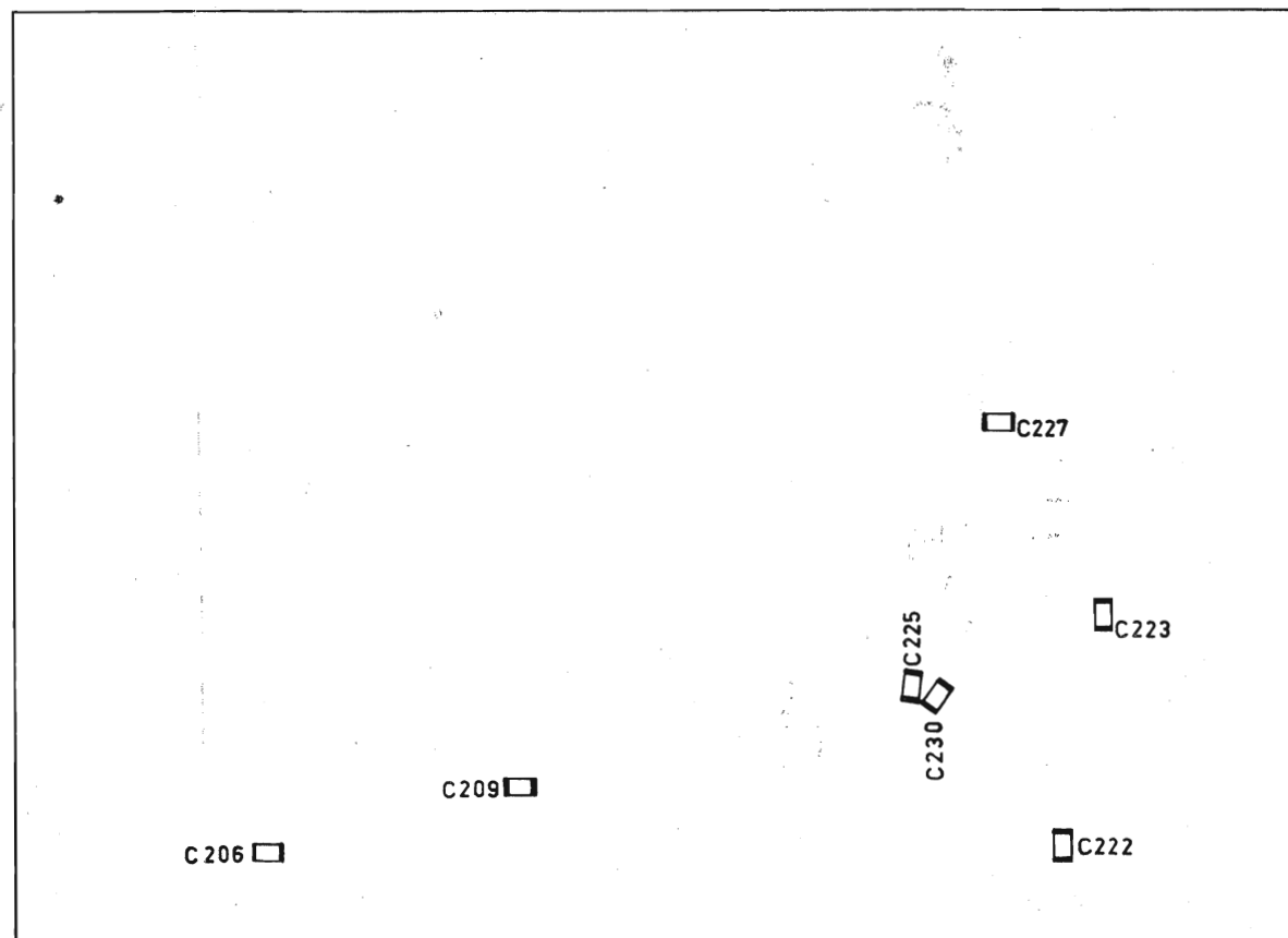
Figure X-10. Component layout prescaler PM 6625, Soldering side
