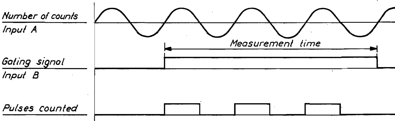
Fig. VI-9. Gated by B measurement
